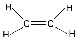
Ethene
